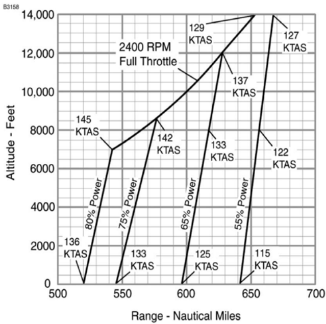
45 MINUTES RESERVE 64 GALLONS USABLE FUEL
