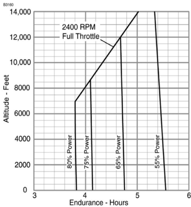
45 MINUTES RESERVE 64 GALLONS USABLE FUEL
