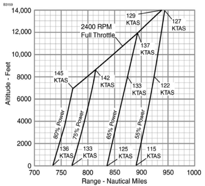
45 MINUTES RESERVE 87 GALLONS USABLE FUEL
